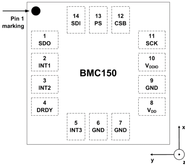
Pin configuration (top view)
