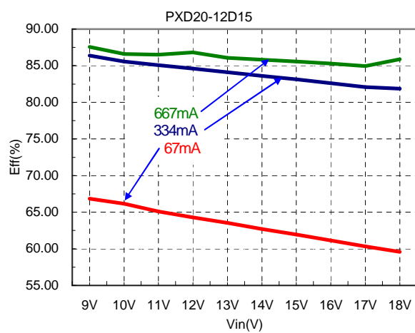
b. Efficiency with line change under different load condition at room temperature
