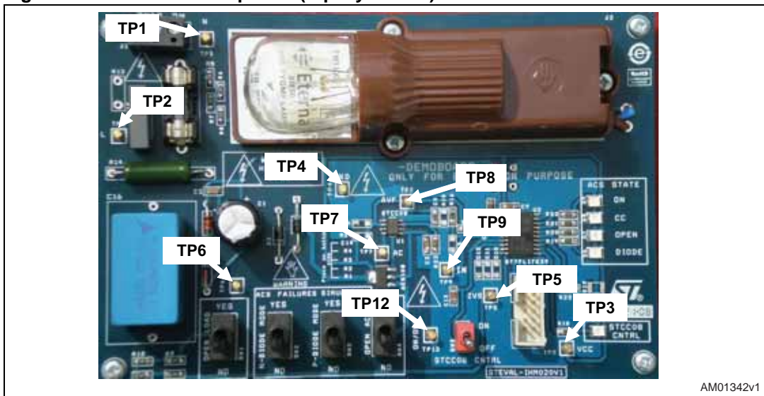
Figure 7. Measurement points (top layer view)
