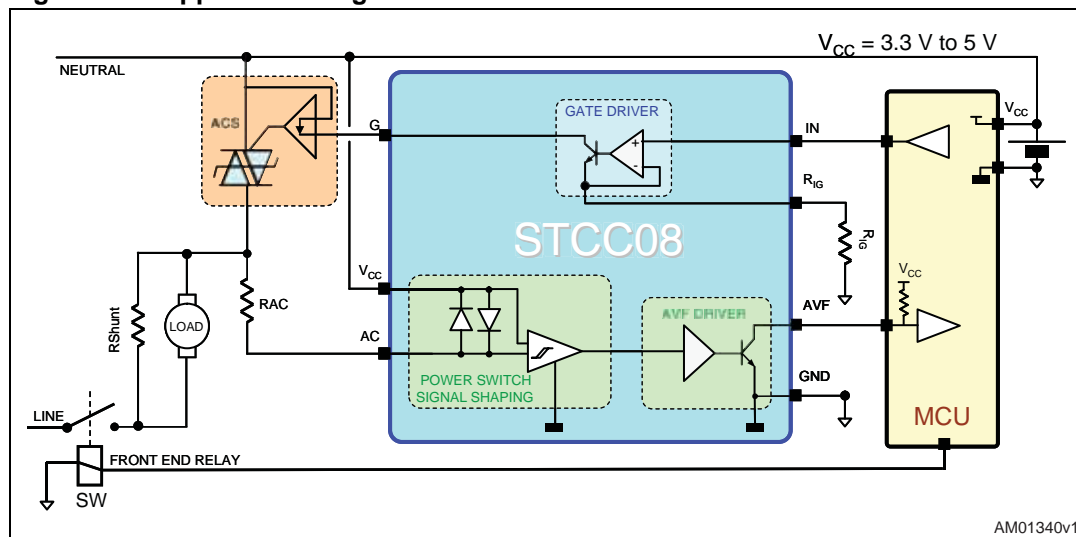
Figure 5. Application diagram
