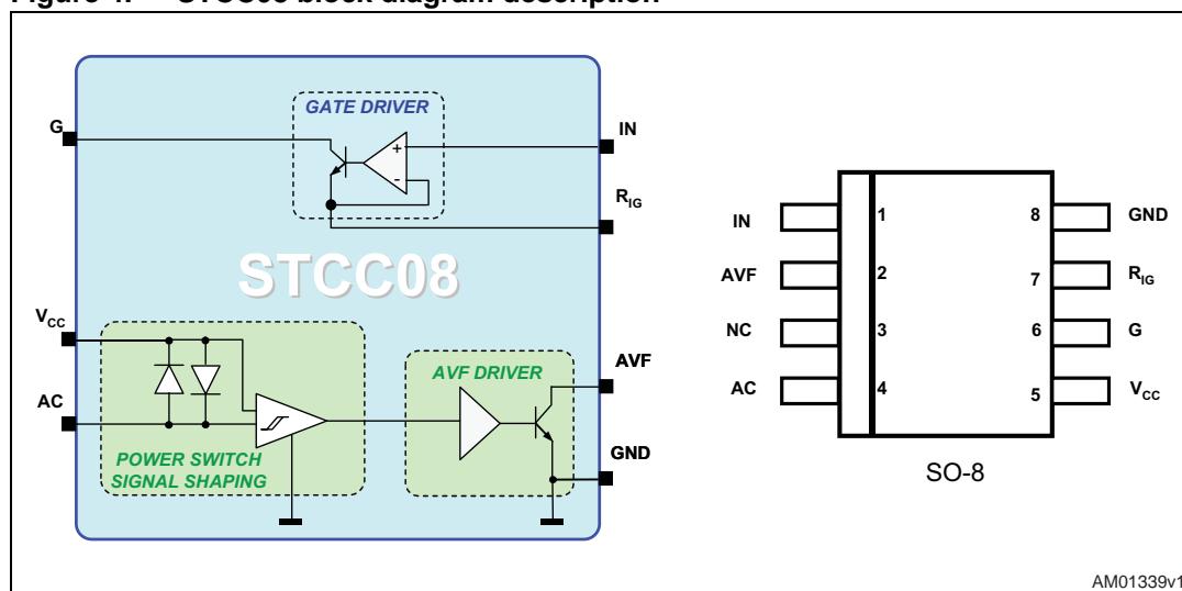
Figure 4. STCC08 block diagram description
