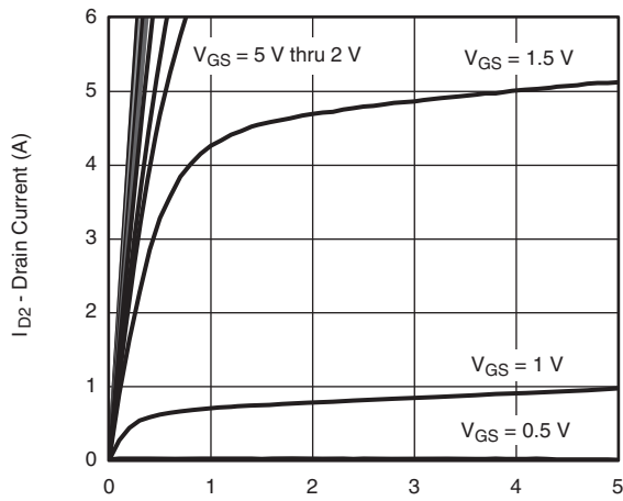
V_{DS2} - Drain-to-Source Voltage (V) Output Characteristics
