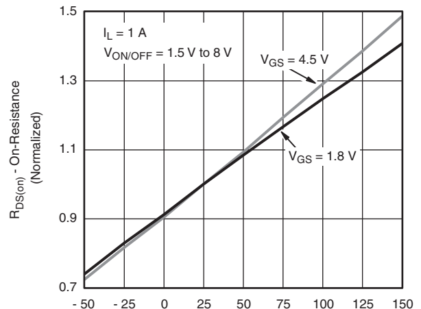
T_J - Junction Temperature (°C) Normalized On-Resistance vs. Junction Temperature
