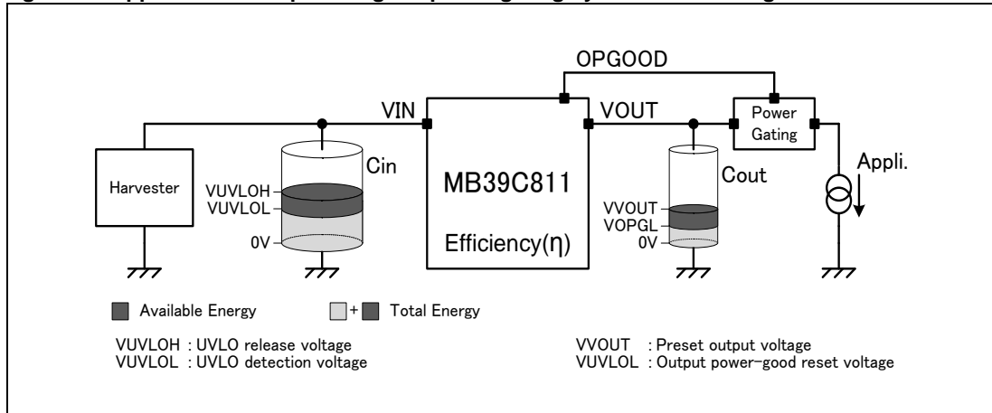
Figure 10. Application example using the power gating by the OPGOOD signal
