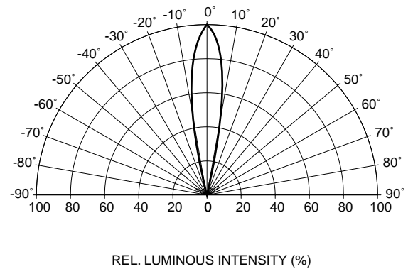
REL. LUMINOUS INTENSITY (%) Fig. 4 Radiation Diagram
