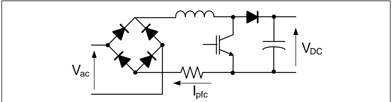
Figure 23 Basic Boost PFC Circuit
