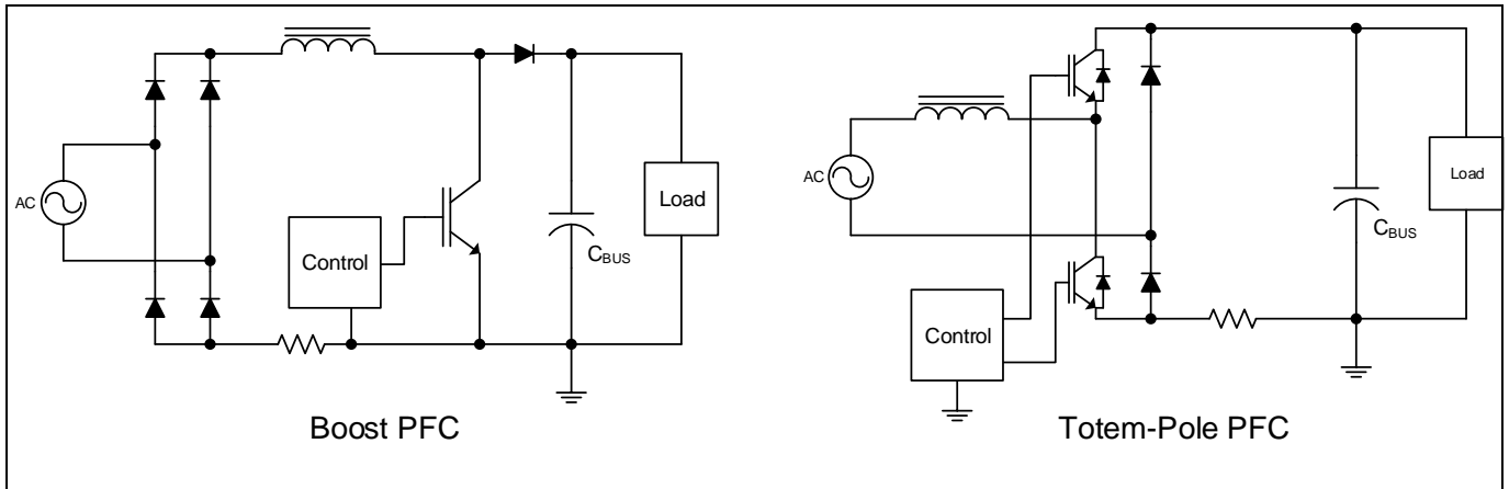
Figure 25 PFC topologies
