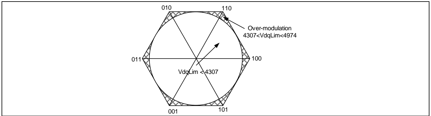
Figure 43 Over modulation
