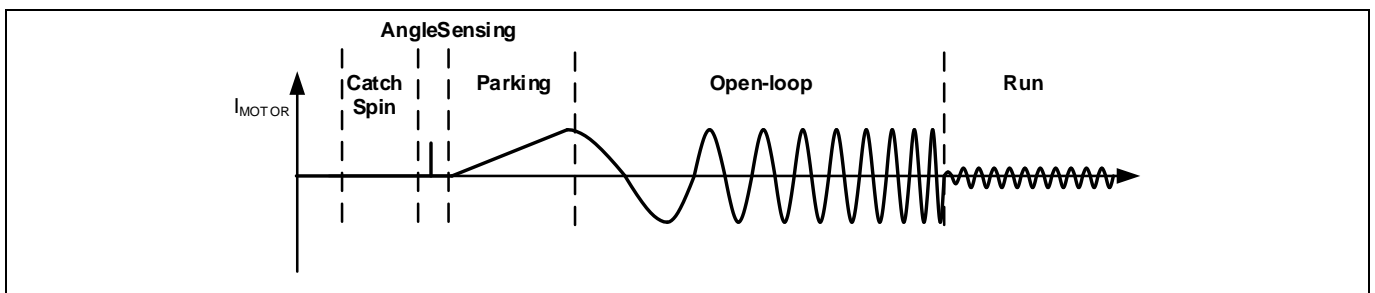
Figure 3 Motor start waveform
