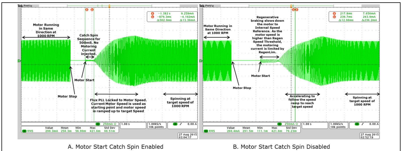
Figure 17 Motor Phase Current Waveform - Forward Catch Spin - Motor start with/without catch
