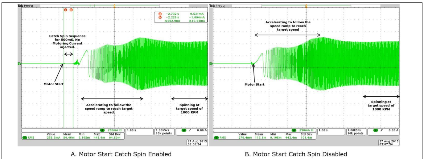
Figure 15 Motor Phase Current - Zero Speed Catch Spin - Motor start with/without catch spin
