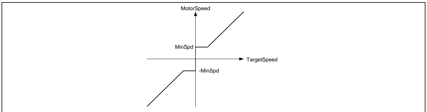
Figure 40 Minimum Speed
