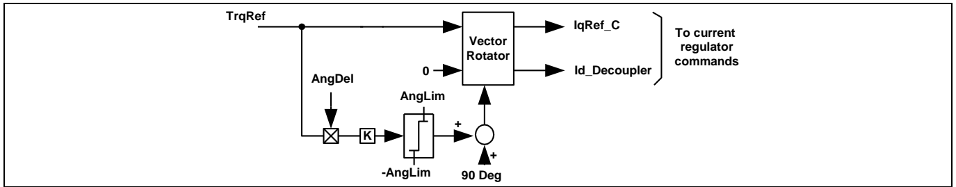
Figure 44 Angle Del
